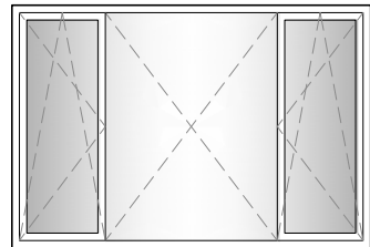
31. 3 SECTION WINDOW 1/4 1/2 1/4 ENDS TILT / TURN CENTRE FIXED IN FRAME (UNEVEN GLASS)
