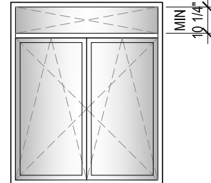
18. DOUBLE SASH TILT / TURN WINDOW WITH FIXED IN FRAME TRANSOM
