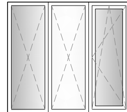
26. 3 SECTION WINDOW 1 SECTION TILT / TURN , 2 SECTIONS FIXED IN FRAME (UNEVEN GLASS)
