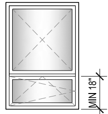
10. 2 SECTION WINDOW BOTTOM SECTION TILT / TURN (MIN. RESTRICTIONS APPLY) TOP FIXED IN SASH GLASS EVEN
