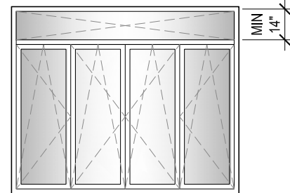
34. 4 SECTION WINDOW ALL SECTIONS TILT AND TURN IN FOR CLEANING WITH 4 SECTION TRANSOM
