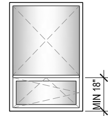
9. 2 SECTION WINDOW BOTTOM SECTION TILT / TURN (MIN. RESTRICTIONS APPLY) TOP FIXED IN FRAME GLASS UNEVEN
