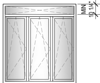
22. 3 SECTION WINDOW ALL SECTIONS TILT AND ALL SECTIONS TURN IN FOR CLEANING WITH FIXED IN FRAME TRANSOM
