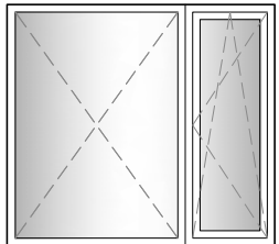
29. 2 SECTION WINDOW 1/3 TILT / TURN 2/3 FIXED IN FRAME (UNEVEN GLASS)
