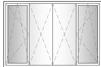
33. 4 SECTION WINDOW 2 SECTIONS TILT / TURN 2 SECTIONS FIXED IN FRAME (UNEVEN GLASS)
