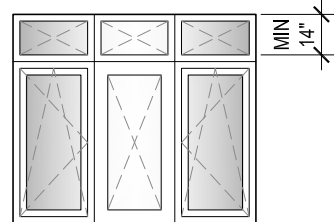
25. 3 SECTION WINDOW 2 SECTIONS TILT / TURN AND 1 SECTION FIXED IN SASH (EVEN GLASS) WITH FIXED TRANSOM
