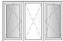
24. 3 SECTION WINDOW 2 SECTIONS TILT / TURN AND 1 SECTION FIXED IN FRAME (UNEVEN GLASS)
