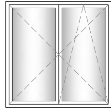
14. NO POST DOUBLE WINDOW RIGHT SIDE TILT / TURN , LEFT SIDE TURN ONLY
