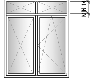
20. 2 SECTION WINDOW 1 SIDE TILT / TURN , 1 SIDE FIXED IN SASH (EVEN GLASS) WITH FIXED IN FRAME TRANSOM
