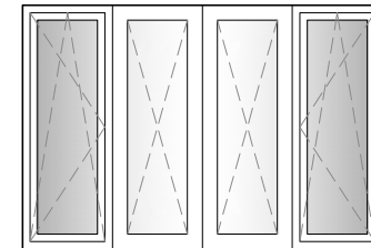
35. 4 SECTION WINDOW 2 SECTIONS TILT / TURN 2 SECTIONS FIXED IN SASH (EVEN GLASS)
