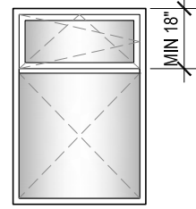
5. SINGLE WINDOW FIXED IN FRAME WITH TILT / TURN TRANSOM (GLASS UNEVEN) MIN RESTRICTIONS APPLY
