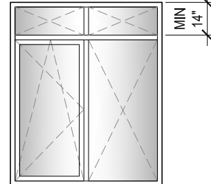
19. 2 SECTION WINDOW 1 SIDE TILT / TURN , 1 SIDE FIXED IN FRAME (UNEVEN GLASS ) WITH FIXED IN FRAME TRANSOM
