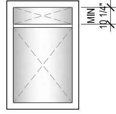
7. SINGLE WINDOW FIXED IN SASH WITH FIXED IN SASH TRANSOM (EVEN GLASS)
