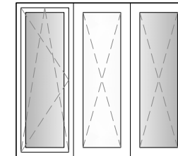
27. 3 SECTION WINDOW 1 SECTION TILT / TURN , 2 SECTIONS FIXED IN SASH (EVEN GLASS)
