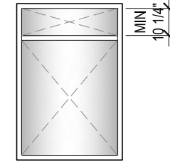
8. SINGLE WINDOW FIXED IN FRAME WITH FIXED IN FRAME TRANSOM (EVEN GLASS)
