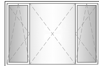
31. 3 SECTION WINDOW 1/2 1/2 1/2 ENDS TILT / TURN CENTRE FIXED IN FRAME (UNEVEN GLASS)
