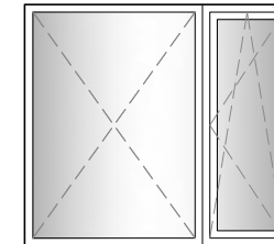
29. 2 SECTION WINDOW 1/3 TILT / TURN 2/3 FIXED IN FRAME (UNEVEN GLASS)
